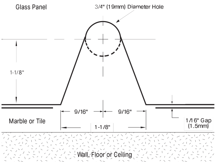
310 WIDE CLIP NOTCH
