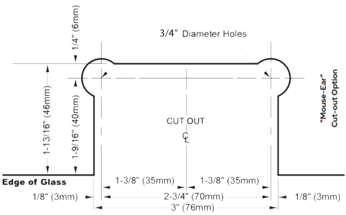
310 HEAVY DUTY HINGE
