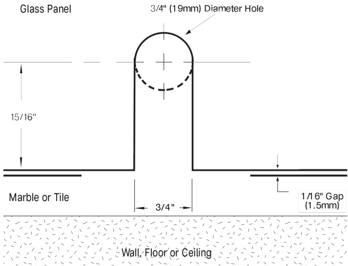
310 15/16" CLIP NOTCH
