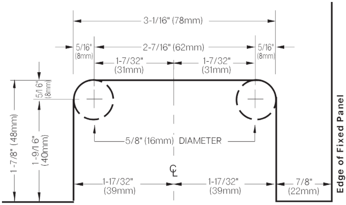
310 HEAVY DUTY HINGE
