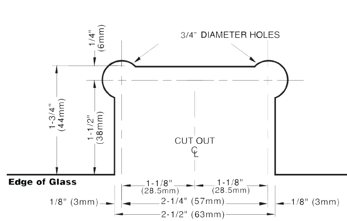
310 STANDARD DUTY HINGE
